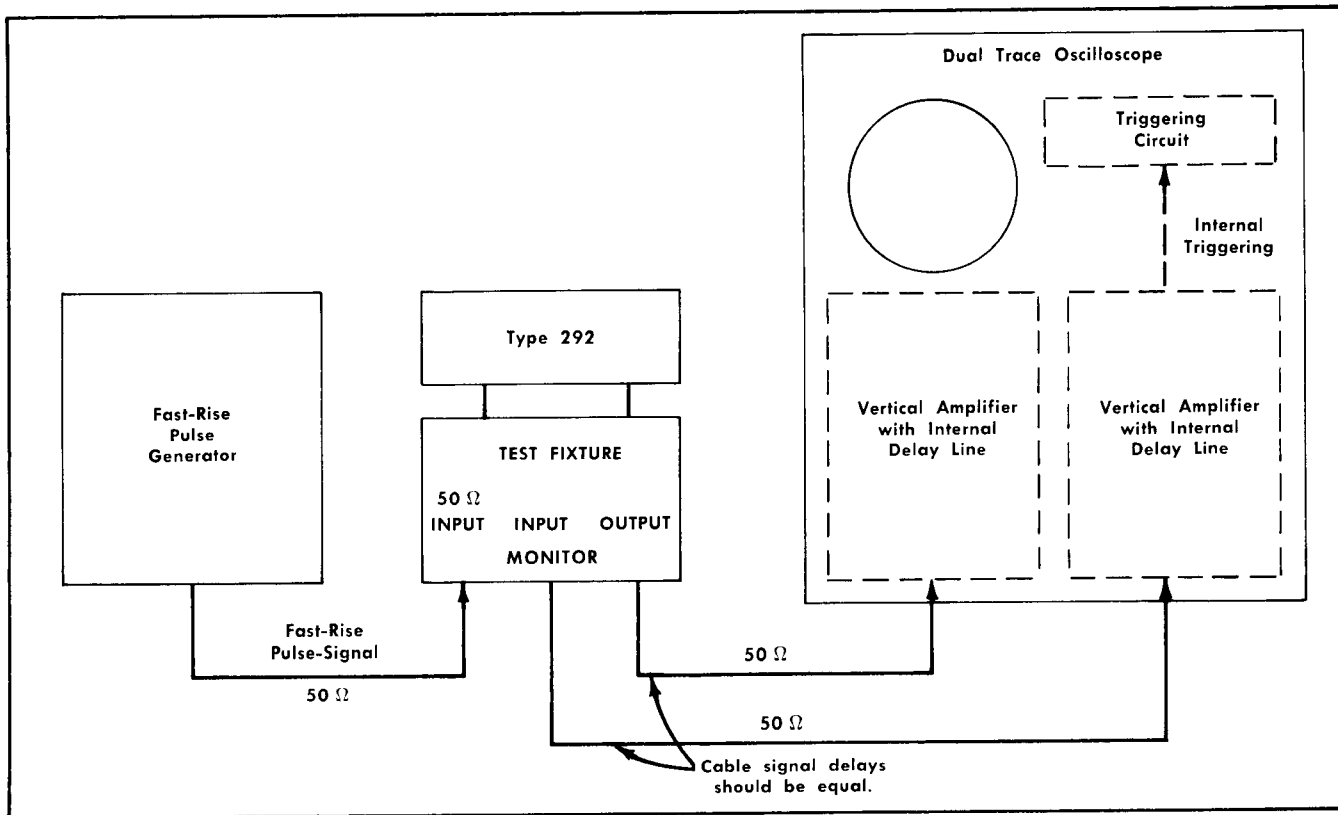
Fig. 2-4. Block diagram of Test System One.
